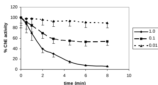
Fig. 1. Inhibition of cholinesterases in the rat blood by different concentrations of sarin in vitro . Sarin concentrations: 0.01–0.1 and 1.0 \mu\text{M} .
